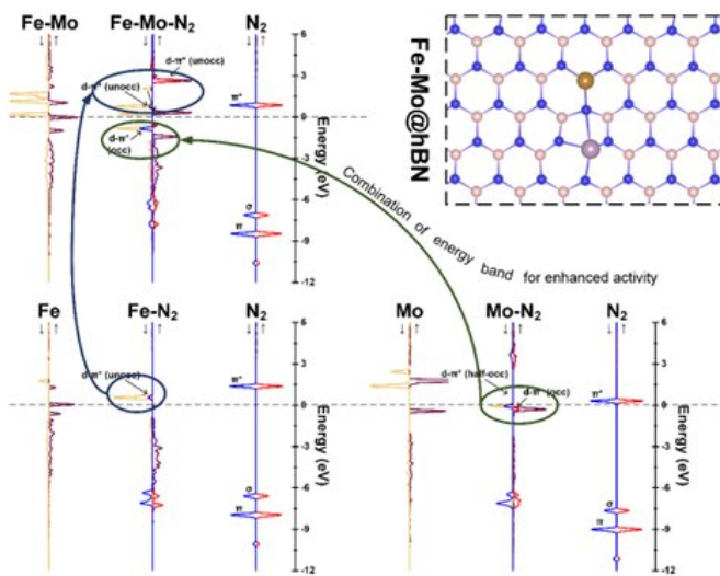
How the heterogeneous catalyst integrates properties of the components to enhance catalytic performance. Credit: Southeast University, China
